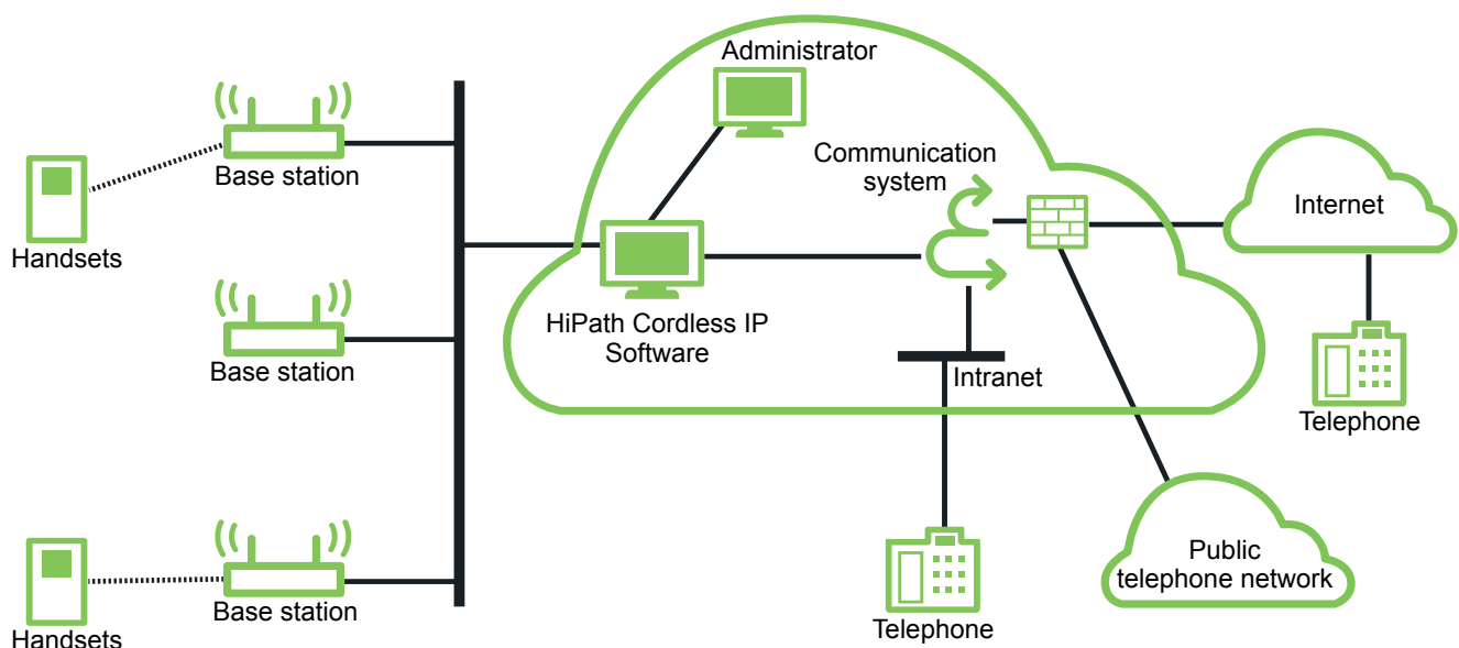
Configuration/System concept
